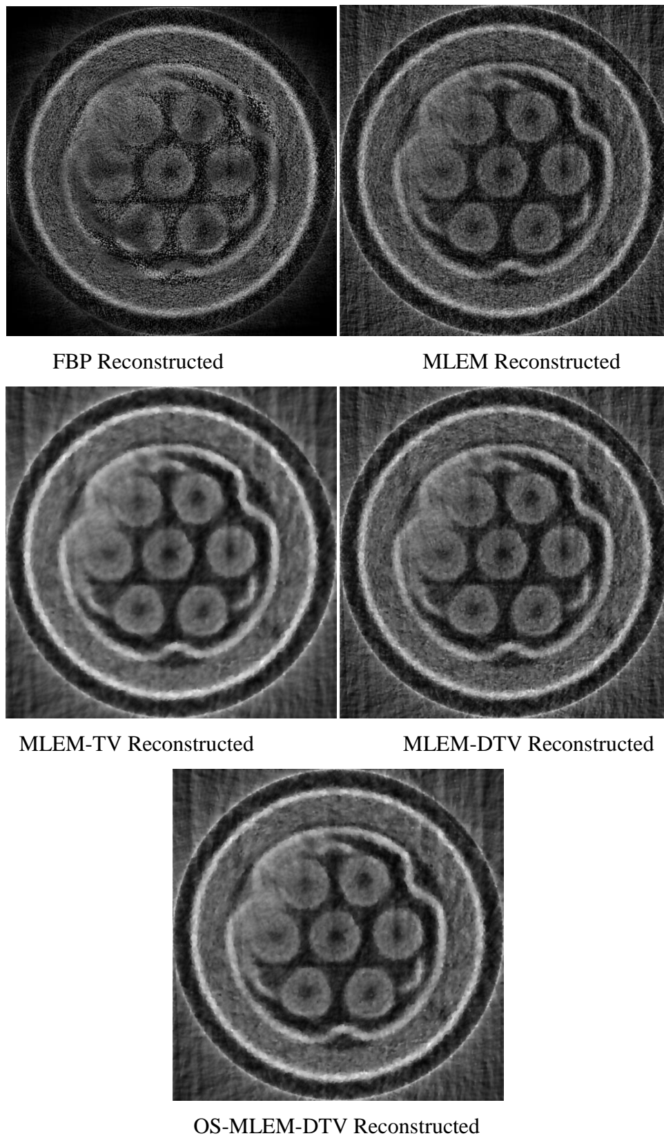
Figure 4.6. Reconstructed image of nuclear fuel using various algorithm methods.
