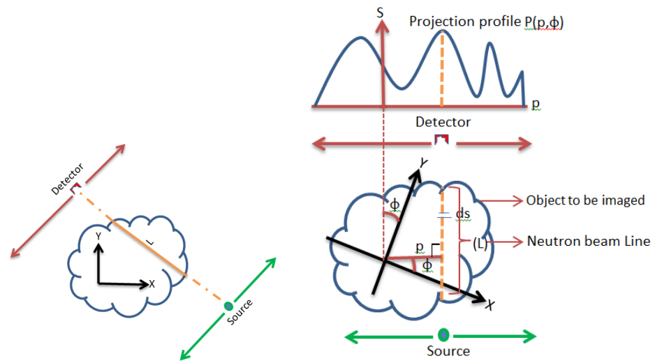
Figure 2.11. Radon transform
