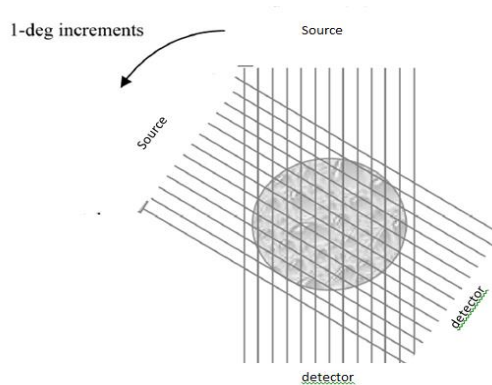
Figure 2.4. Method of acquiring projections[9]
